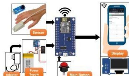
Figure 1 Tool block diagram
