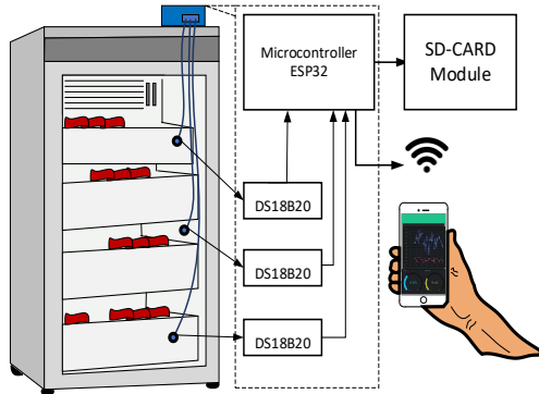
FIGURE 1. The diagram block
