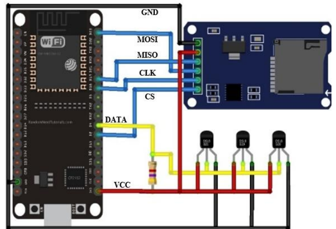
Figure 3. All Circuit blood bank
