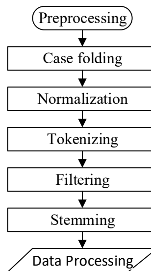
FIGURE 3. Data Preprocessing
