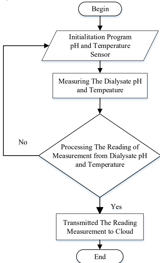
FIGURE 2. The flowchart of Arduino process
