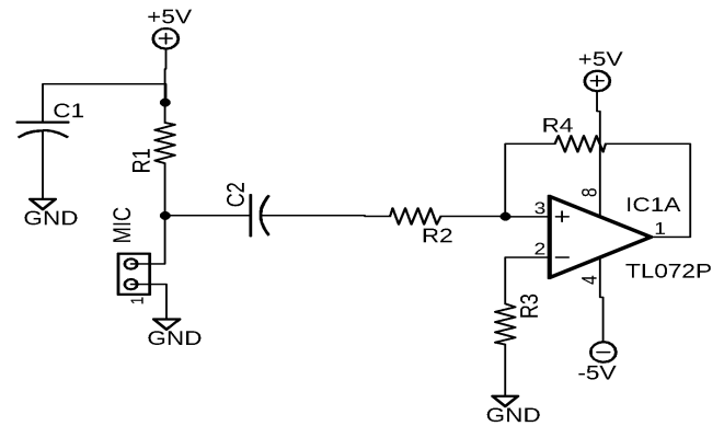
(pre amplifier)
