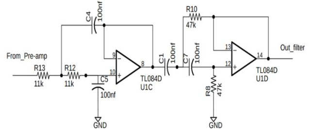
(band pass filter)
