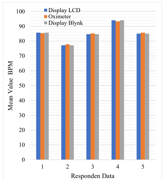
FIGURE 3. There are 3 BPM reading diagrams in each respondent, namely readings on LCD Displays, Oximeters and Blynk Displays
