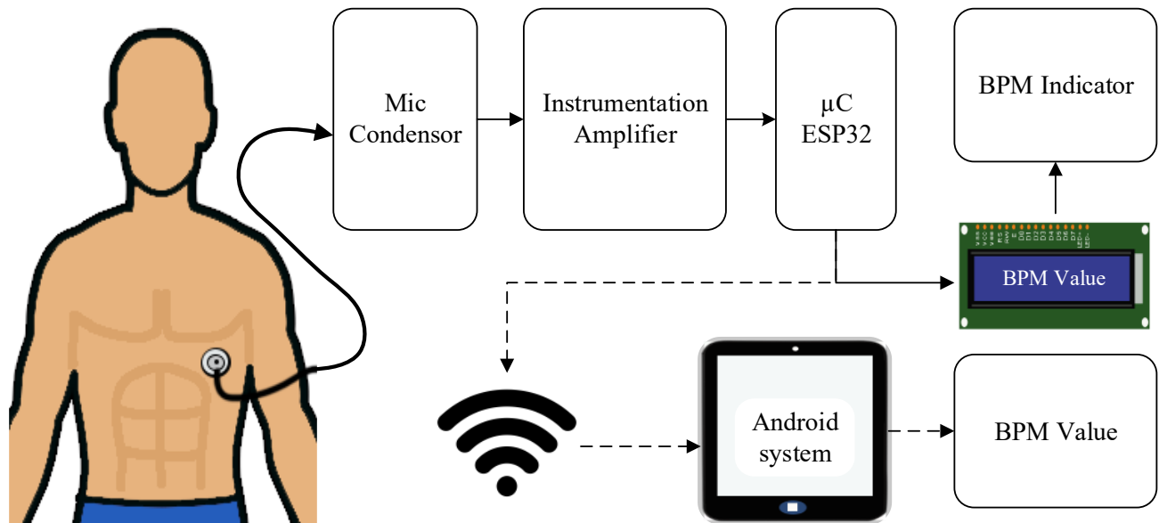
FIGURE 1. Block diagram, the signal output from the condenser mic will be filtered using a signal conditioning circuit then processed in the ESP32 microcontroller which will be displayed on the LCD and sent via the blynk application to the android system.
