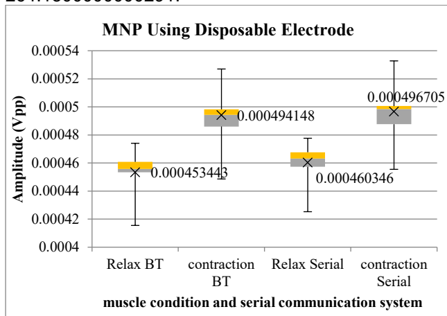
FIGURE 11. Boxplot of mean power value (MNP) with Disposable electrode
