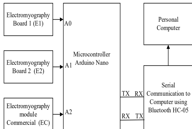
FIGURE 5. Block Diagram Circuit Design Research
