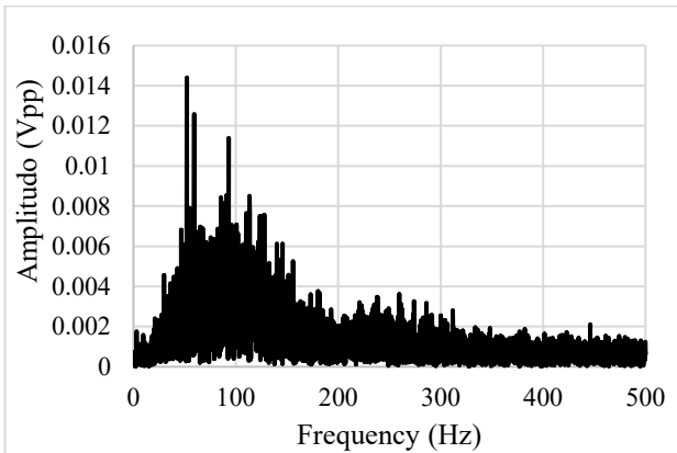
FIGURE 8. Fast Fourier Transform (FFT) results in contraction conditions
