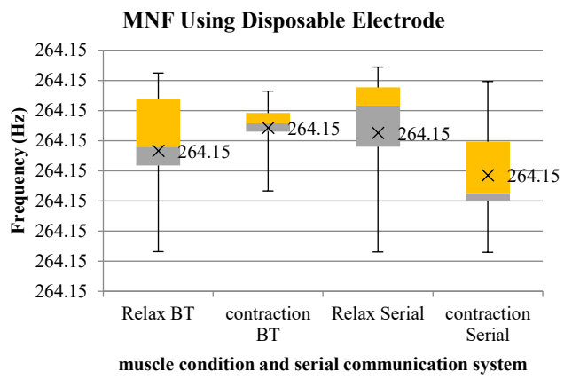
FIGURE 9. The boxplot of the mean frequency value (MNF) with the Disposable electrode
