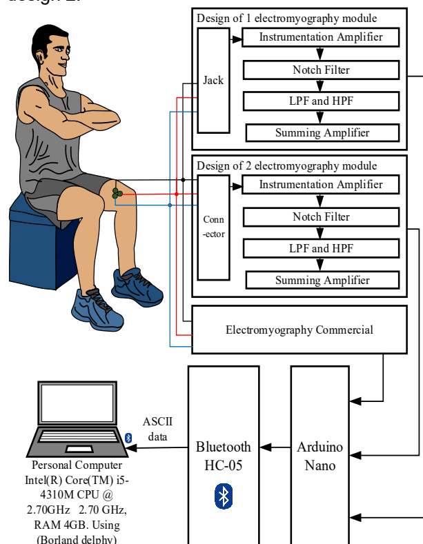
FIGURE 3. Block diagram with detection of the Vastus Medialis muscle
