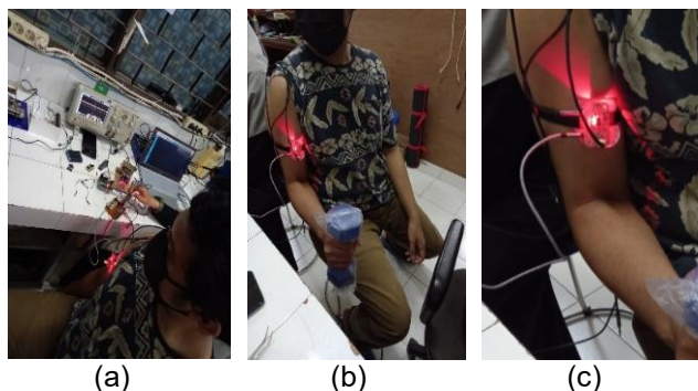
FIGURE 4. (a) Data collection, (b) lifting a barbell while making a 90° turn and (c) Biceps muscle electromyography measurement point
