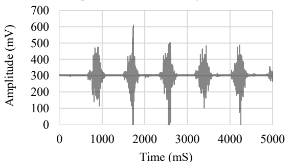
FIGURE 8. Disposable Electrode Design EMG commercial
