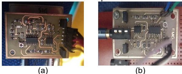
FIGURE 3. Electromyography Design 1 (a) and Electromyography Design 2 (b)
