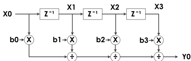
FIGURE 1. Transfer function digital filter
