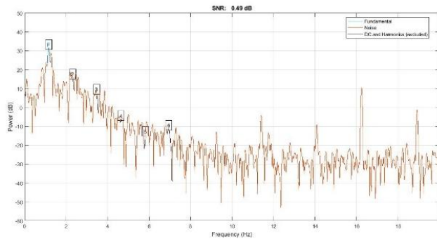
FIGURE 9. SNR Test using Adaptive LMS Filter in Relaxed Conditions. the blue chart is fundamental, red is noise and DC harmony is displayed in black
