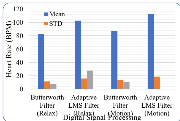
FIGURE 6. Comparison between Butterworth filter and Adaptive LMS filter with two conditions, namely relaxed condition and motion condition.
