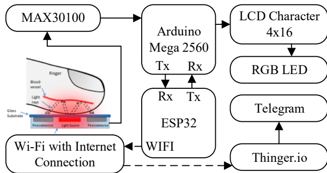
FIGURE 1 Diagram Blok
