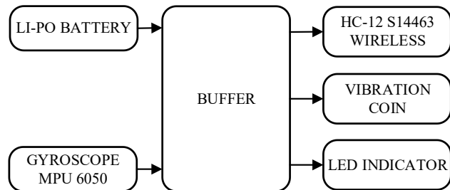
FIGURE 1. The Block Diagram of Gyroscope Bracelet
