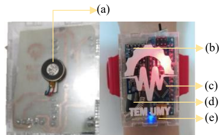
FIGURE 5. Congregation's Device. (a) indicates vibration coin, (b) indicates wireless HC12, (c) Arduino NANO, (d) Battery, and (e) LED Indicator
